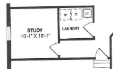
FIRST FLOOR WITH OPTIONAL DEN/LAUNDRY LAYOUT
